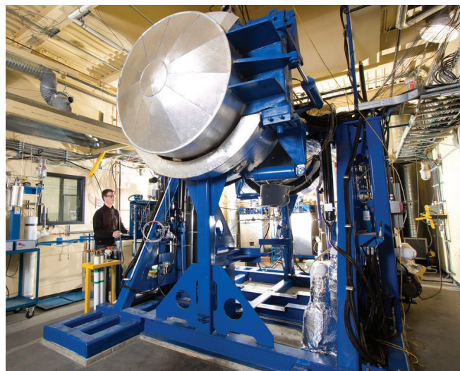
Large 3-D physical model
