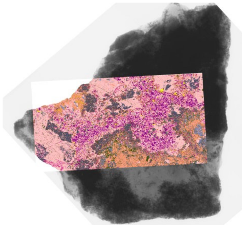
Illustration of mineral map determined by QEMSCAN®; registering with greyscale values obtained from 2-D micro-CT imaging, where darker areas represent high-density rare earth minerals.
