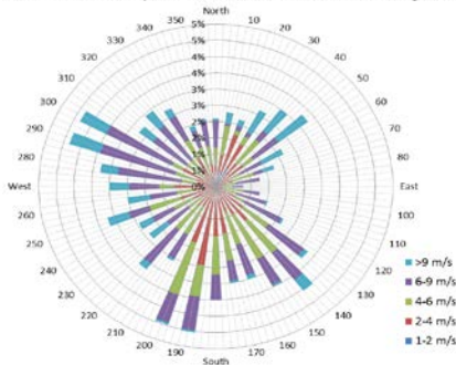
1/2 hr Maximum Wind Speed and Direction Saskatoon August 2018
