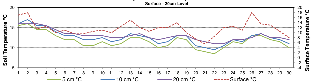
Soil Temperatures for September 2023
