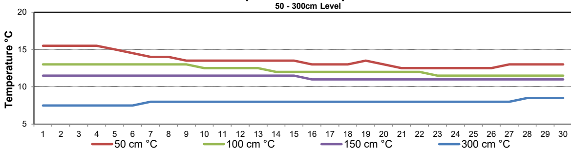
Soil Temperatures for September 2023
