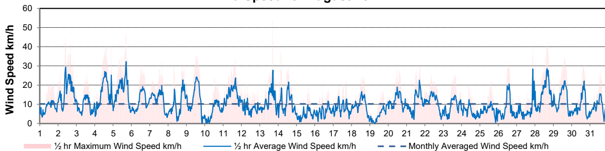
Wind Speed for August 2022
