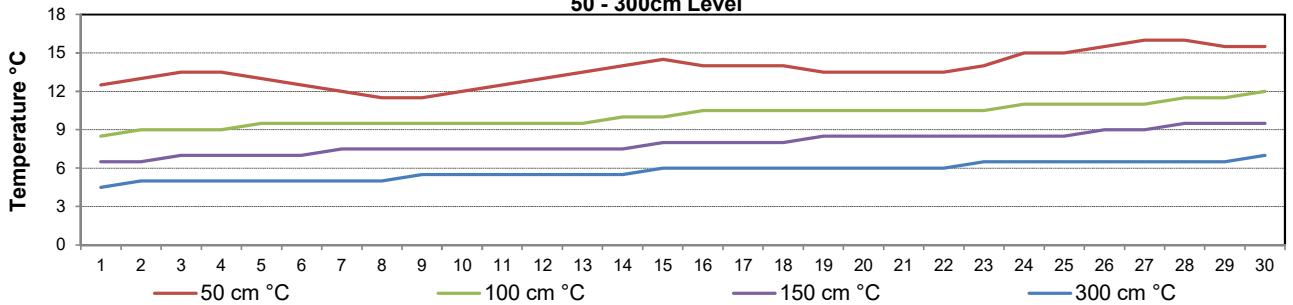
Soil Temperatures for June 2020 50 - 300cm Level
