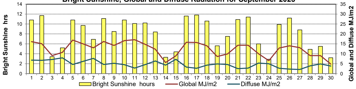
Bright Sunshine, Global and Diffuse Radiation for September 2025
