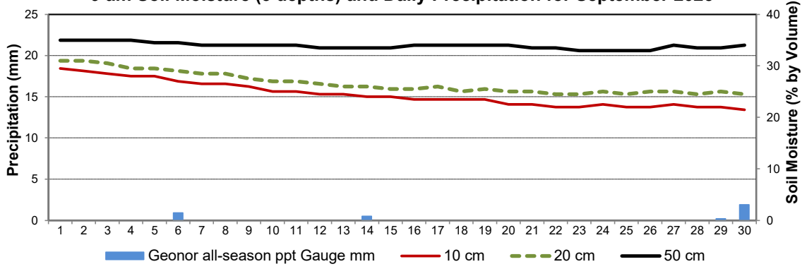
9 am Soil Moisture (3 depths) and Daily Precipitation for September 2025
